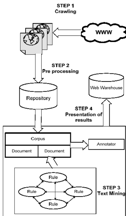
Fig. 2 The Web Text Mining Process
