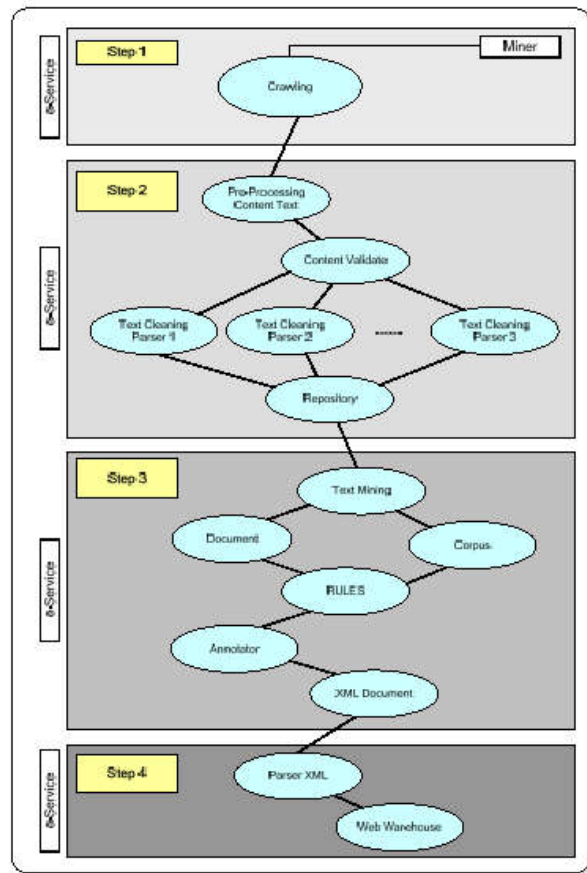
Fig. 6. E-service Workflow in Web Text Mining Process
