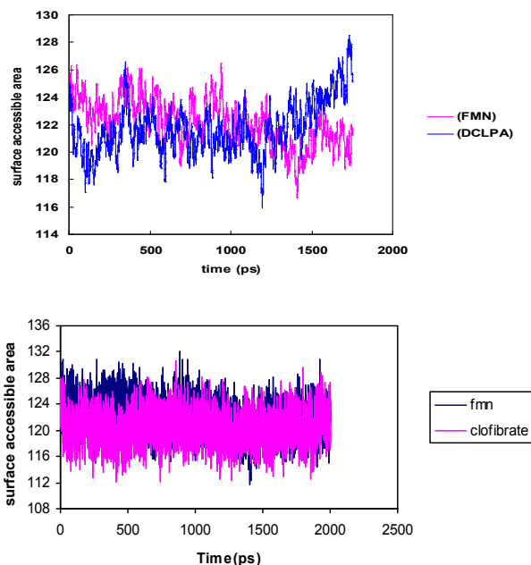
Fig. 3. Accessible surface of the simulated enzyme
