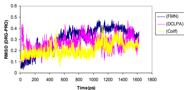
Fig. 2. RMSD variations of inhibitors in simulated system
