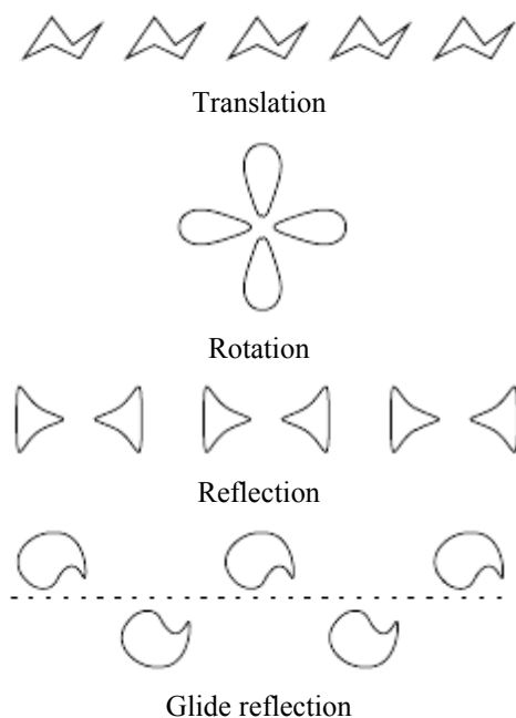
Fig. 1: Transformation rules
