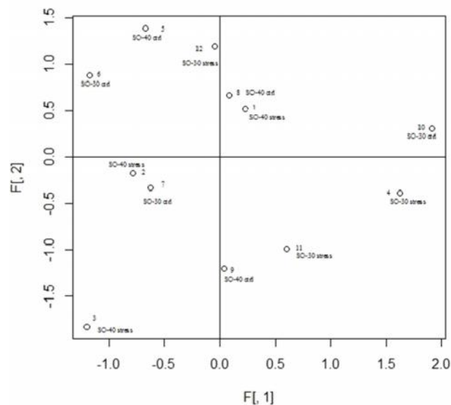
Figure 3. Plot of Principal Components 1 and 2. Note that SO-30 stress treatments tend to be high on PC1
