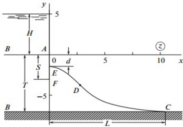
Fig. 1. Flow pattern calculated at \varepsilon=0.6, h_c=0.5, T=7, S=3, and H=5 .
