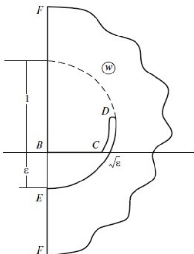
Fig. 2. Regular of complex velocity w for Scheme 1
