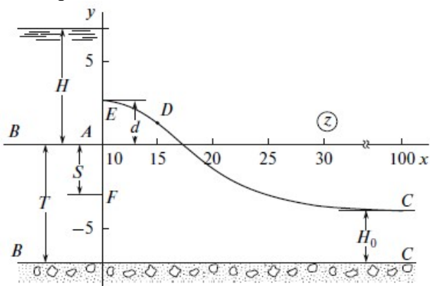
Fig. .3 Flow pattern calculated at \varepsilon = 0.6 , T = 7 , S = 3 , H = 7 , H_0 = 3 , and x_c = 100 .
