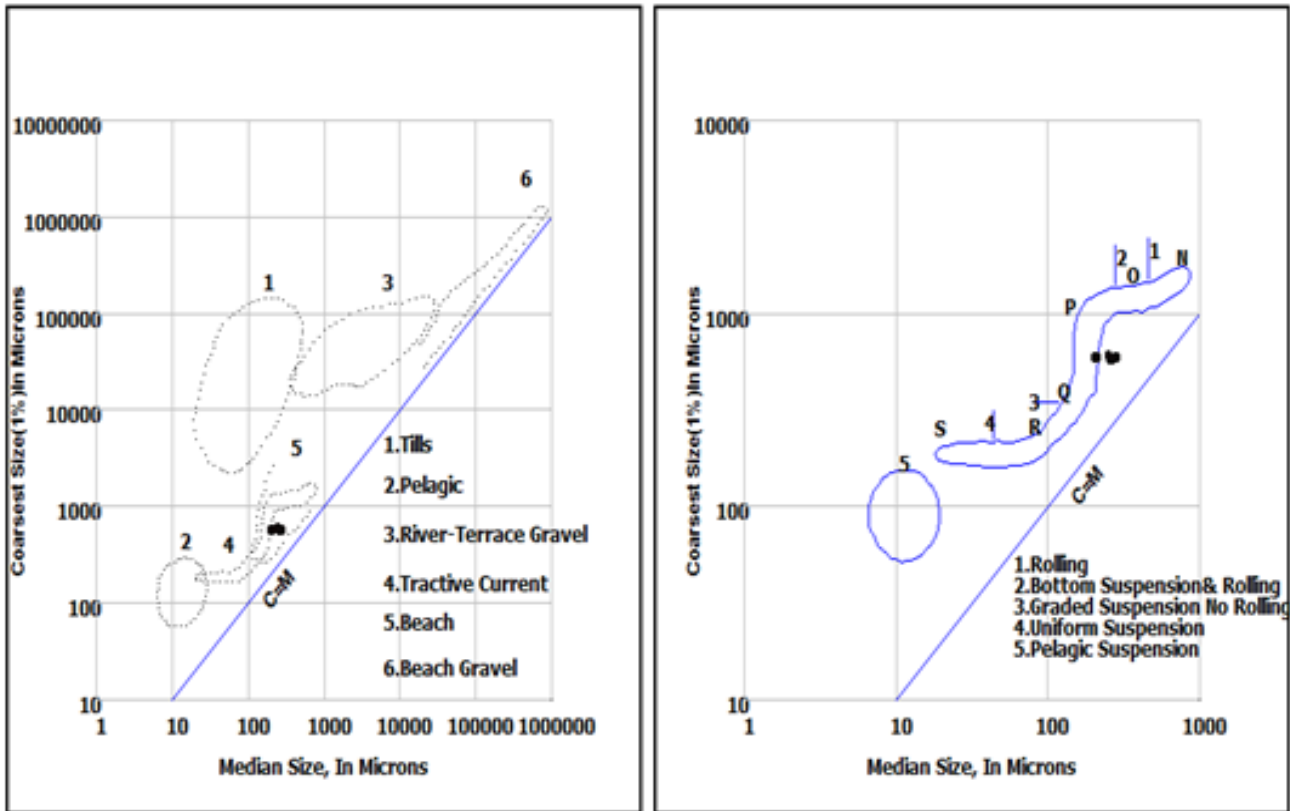
Fig. 6. CM diagram (Passega 1957, 1964) and tractive current deposit plot for Monsoon
