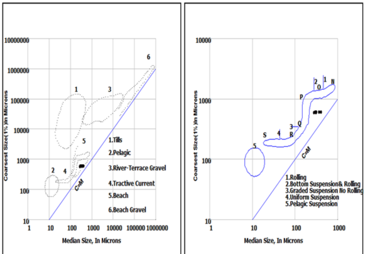
Fig. 5. CM diagram (Passega 1957, 1964) and tractive current deposit plot for Pre monsoon
