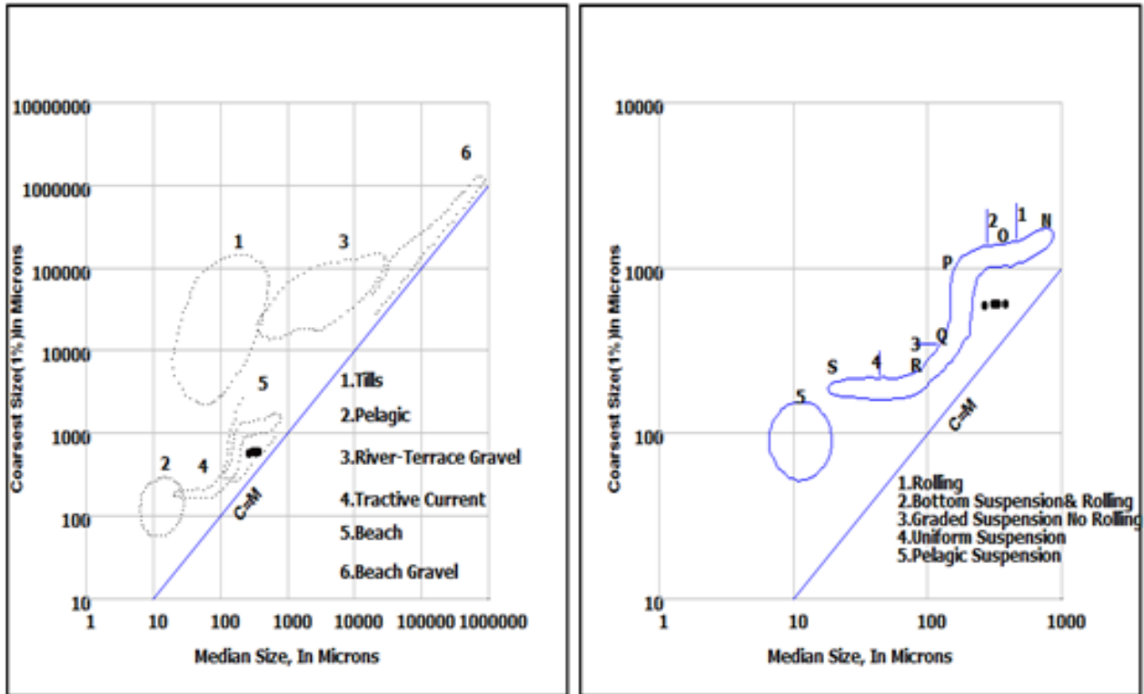
Fig. 7. CM diagram (Passega 1957, 1964) and tractive current deposit plot for Post monsoon
