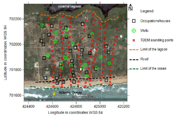
Fig. 5. TDEM soundings on the study area
