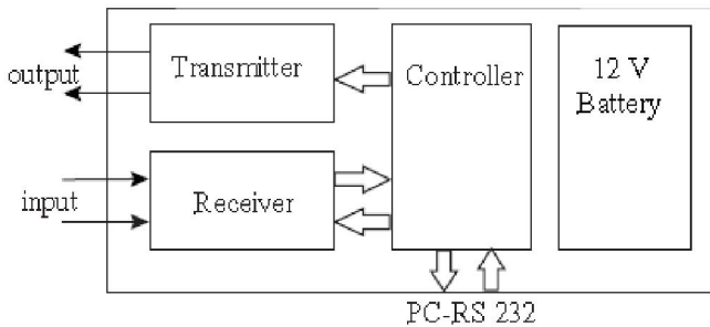
Fig. 4. Block diagram of the TEM-fast 48 device. Modified AEMR (2002a) [1]
