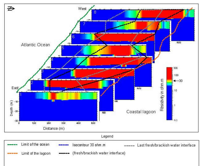
Fig. 7. Lateral extent variation of freshwater lens in dry season
