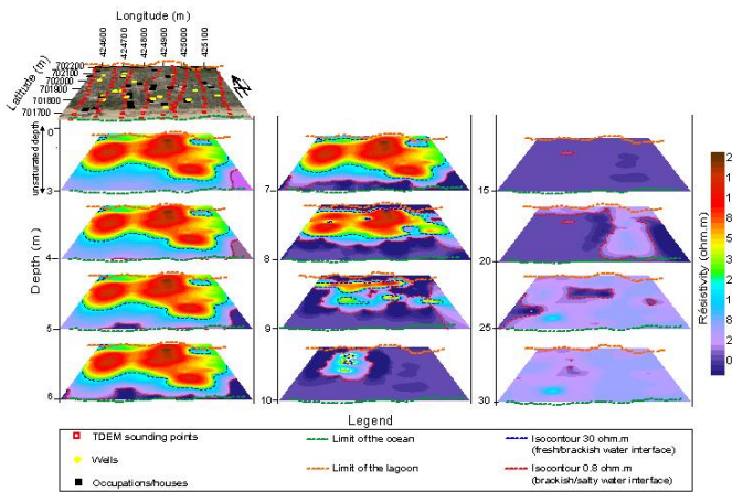
Fig. 9. Depth of freshwater lens (red, yellow and green) in dry season
